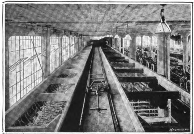
Fig. 7—The Palmer-Bee Co., of Detroit, Mich., installed conveyors and other equipment for handling work at the plant of the Paige-Detroit Motor Car Co. A rack was designed for storing automobile bodies, over which they are carried by a special elevating truck
